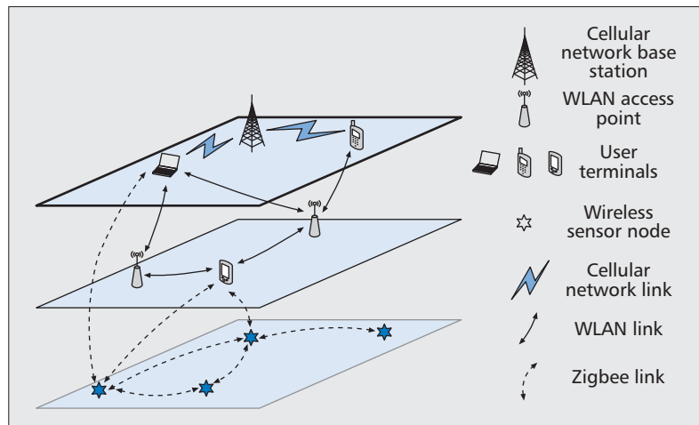
Figure 1. A typical mobile converged network.
