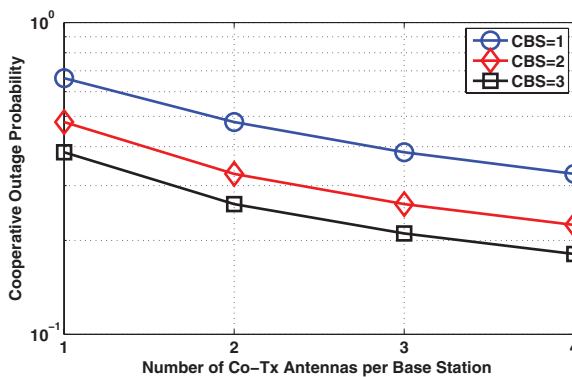
FIGURE 3. The impact of the number of Co-Tx antennas per cooperative BS on the cooperative outage probability.
